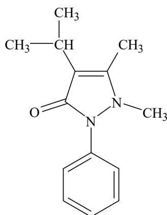
8. Isopropylantipyrine
