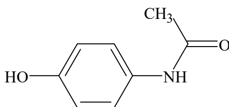
2. Acetaminophen
